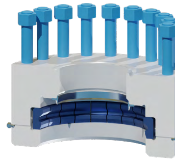
NT-2 Adapter
